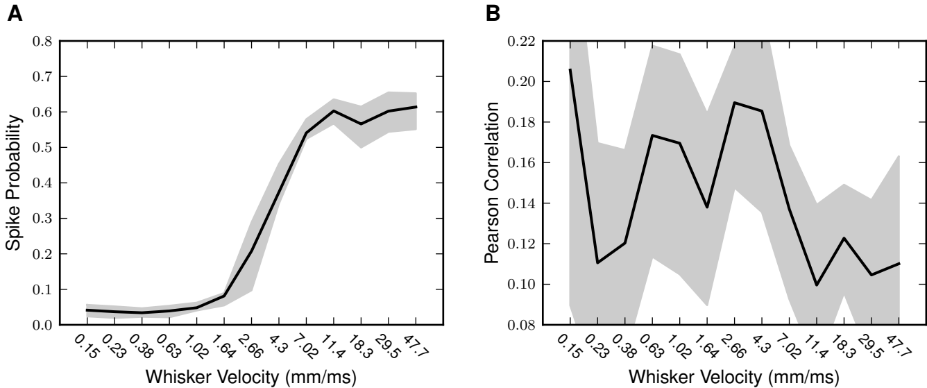
Figure 3: Mean firing rate and correlation coefficients for the data. The mean probability of observing a spike in the 10–15ms post stimulus window considered is shown (panel A ) as a function of the whisker velocity stimulus. Black line shows mean spike probability across the 8 cells considered; grey region shows 25 th -75 th percentile. The Pearson correlation coefficients of neural responses for each stimulus are also shown (panel B ). Black line shows mean correlation coefficient across the 28 pairs among the 8 cells considered; grey region shows 25 th -75 th percentile.
