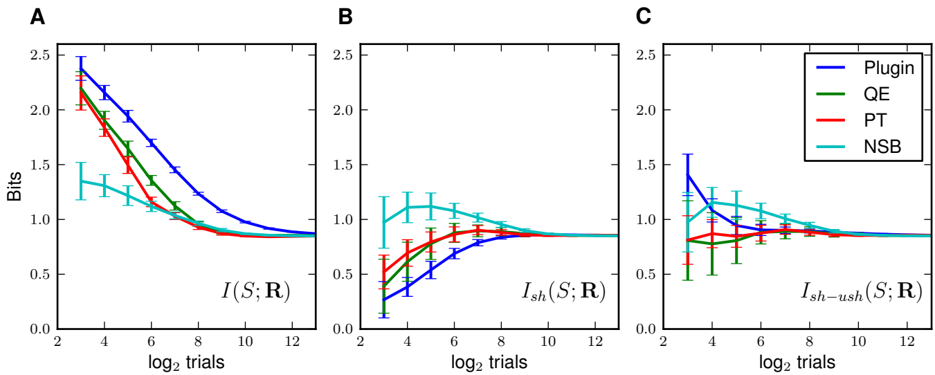
Figure 2: Bias corrected mutual information estimates. The effect of different entropy bias correction methods on the mutual information estimators I (panel A ), I_{sh} (panel B ) and I_{sh-ush} (panel C ) are shown. Data is generated from the same 8 cell model system as in Figure 1. Each point represents the average over 50 simulations of the system; error bars show \pm 1 SD.
