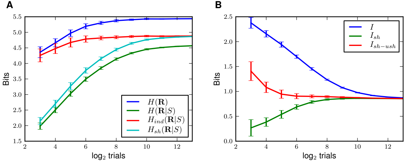
Figure 1: The limited sampling bias. Plugin estimates of entropy quantities (panel A ) and mutual information estimators (panel B ) are shown as function of number of trials per stimulus used for the estimation. Data is generated from a model of 8 cells from rodent somatosensory cortex, responding to whisker stimulation at 13 different velocities (ranging between 0.15 mm/s and 47.7 mm/s). Stimulus-conditional individual and pairwise marginal probabilities are equal to those observed experimentally (see Section 5) but no higher order correlations are present. Each point represents the average over 50 simulations of the system; error bars show \pm 1 SD.
