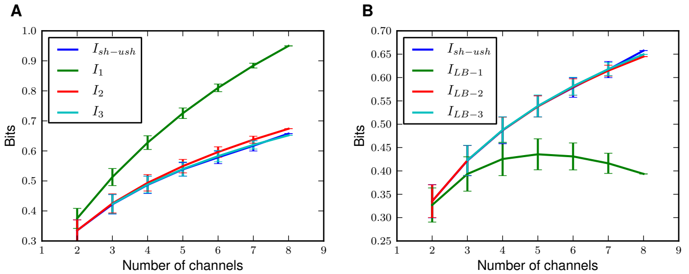
Figure 4: Quantifying the effect of correlations on information. The information I_k(s; \mathbf{R}) carried by systems containing correlations only up to order k , and shortened as I_k ( k = 1, 2, 3 ) (panel A ), lower bounds on information available to a decoder neglecting correlations of order higher than k , I_{LB-k} ( k = 1, 2, 3 ) (panel B ) and the I_{sh-ush} mutual information estimator are shown as a function of the number of cells considered. 8 channels from the experimental data set (see Section 5) were chosen; each point shows the mean value over all \binom{8}{c} combinations of c channels. Error bars show \pm 1 SD. All values are corrected using quadratic extrapolation.
